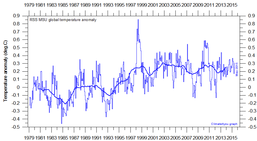
RSS (lower troposphere)
