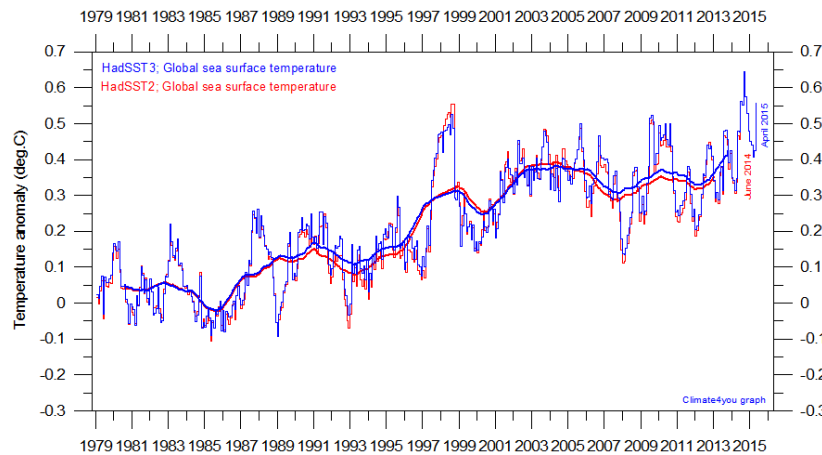
HadSST (ocean surface only)
