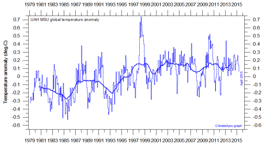
UAH (lower troposphere)
